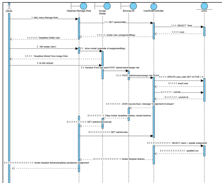
Gambar 3. 37 Sequence Diagram Assign Role
