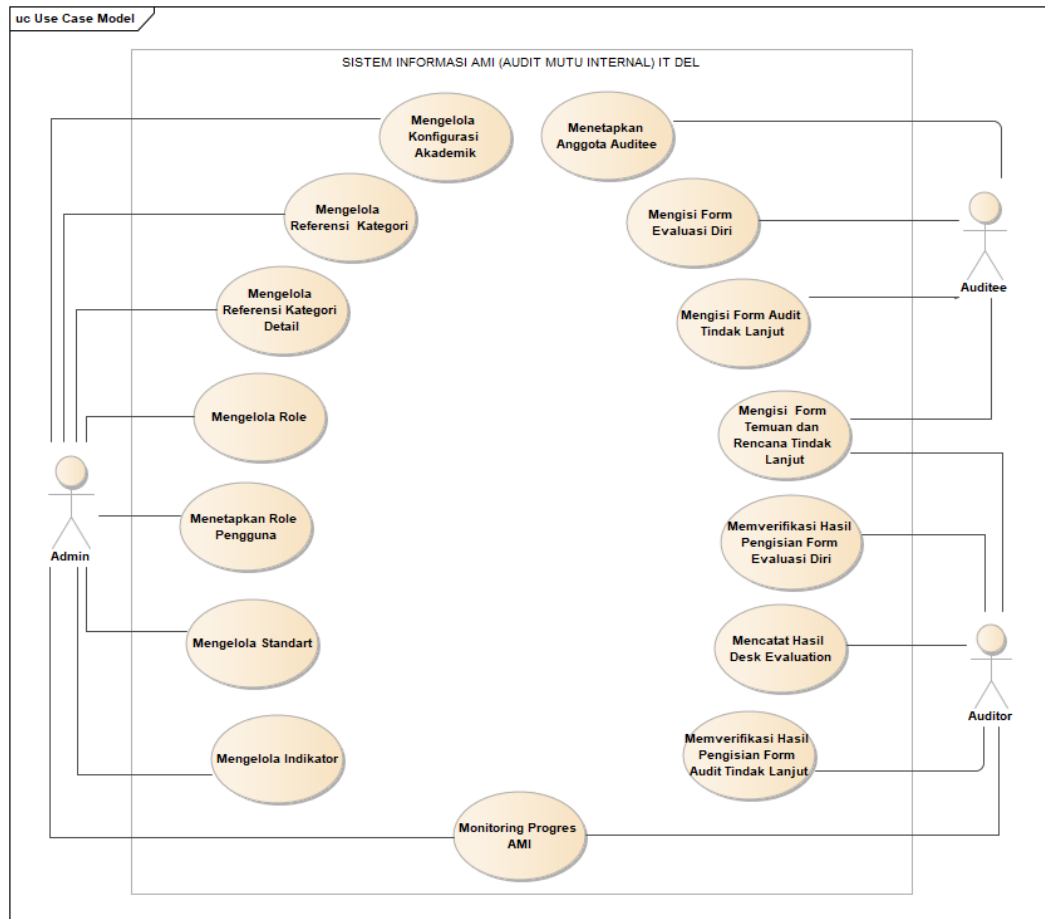
Gambar 3. 30 Use Case Diagram
