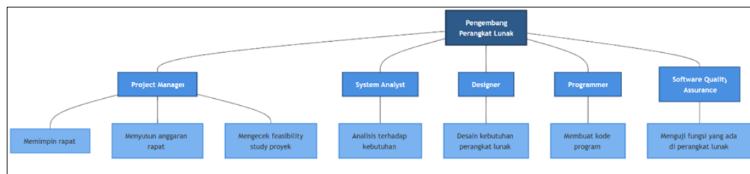
Gambar 2.1 Project organization
