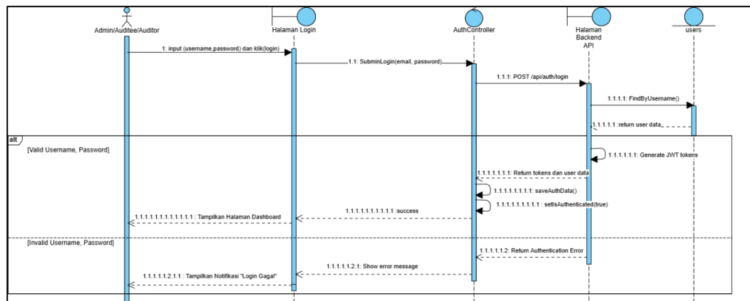
Gambar 3. 32 Sequence Diagram Login
