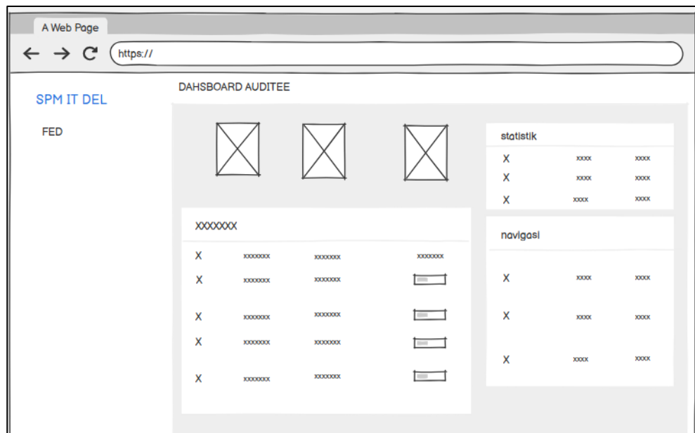
Gambar 3. 56 Wireframe Halaman Dashboard Auditee
