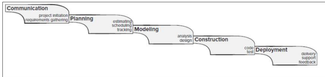
Gambar 1. 2 Metodologi Waterfall
