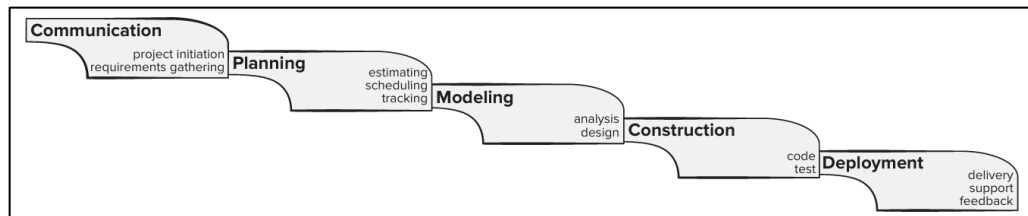
Gambar 2. 2 Metodologi Waterfall
